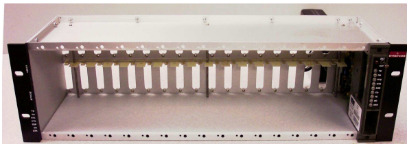
RA-1C.24, RA-1C.21, and RA-1C.35 Rack Adapter
